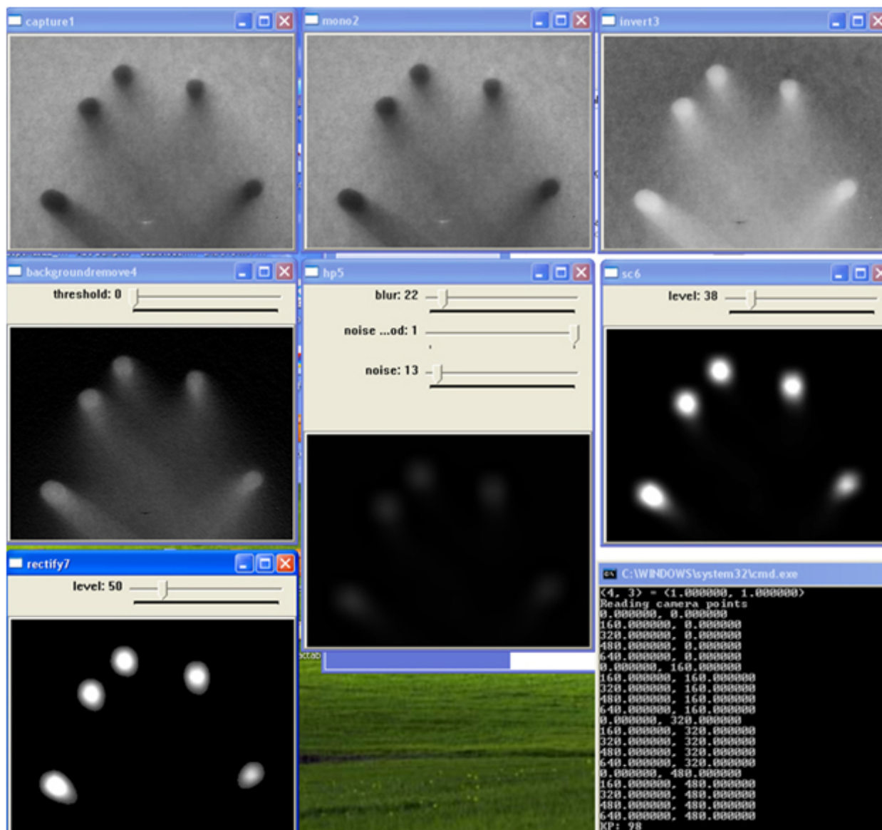
Figure 2. Touchlib Configapp
